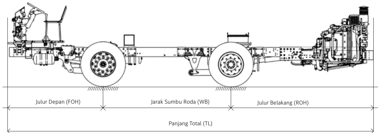
Tampak Samping
