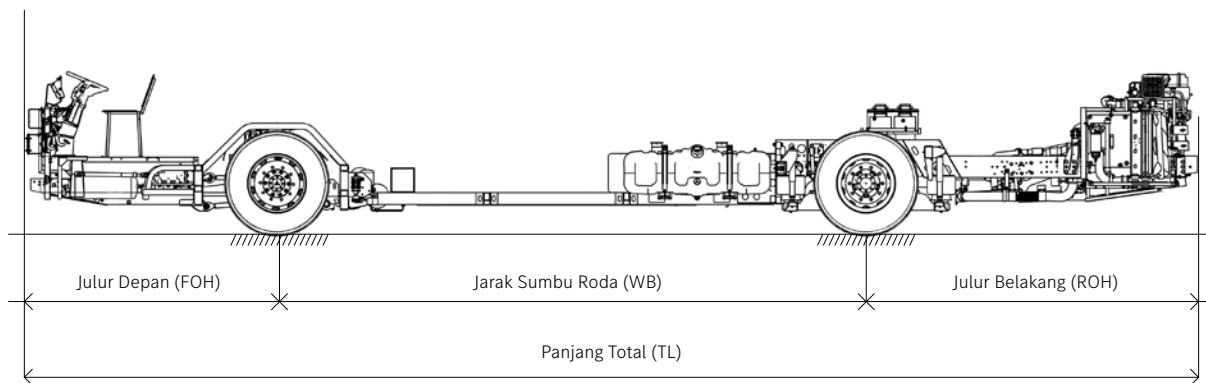
Tampak Samping
